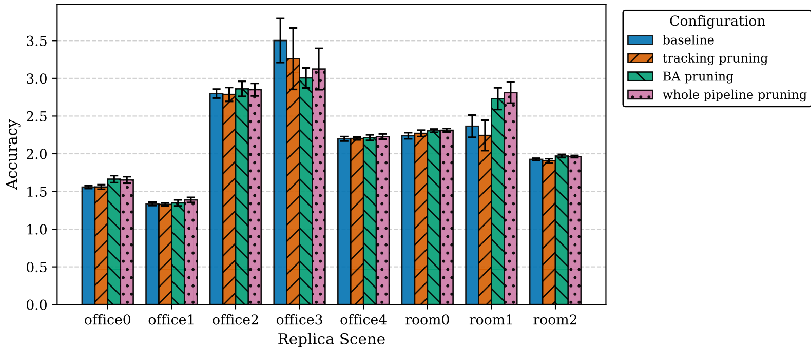
Accuracy ( \downarrow ) across Replica Scenes (Mean & Std Dev)
